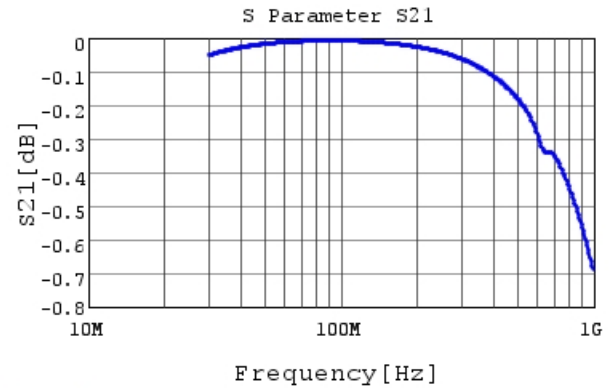
RHE5G2A471J0K1H03B S21 DCOV, 25degC
