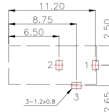
PCB.WELDING DRAWING (TOLERANCE:±0.05)
