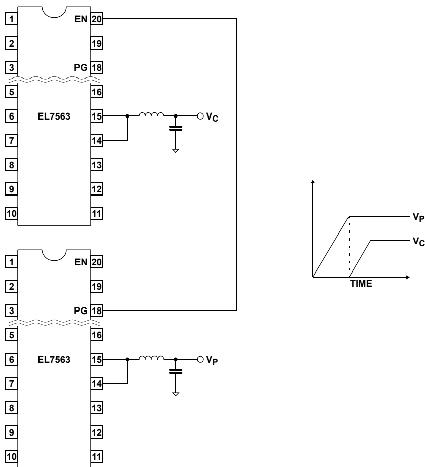
FIGURE 25. OFFSET TRACKING
