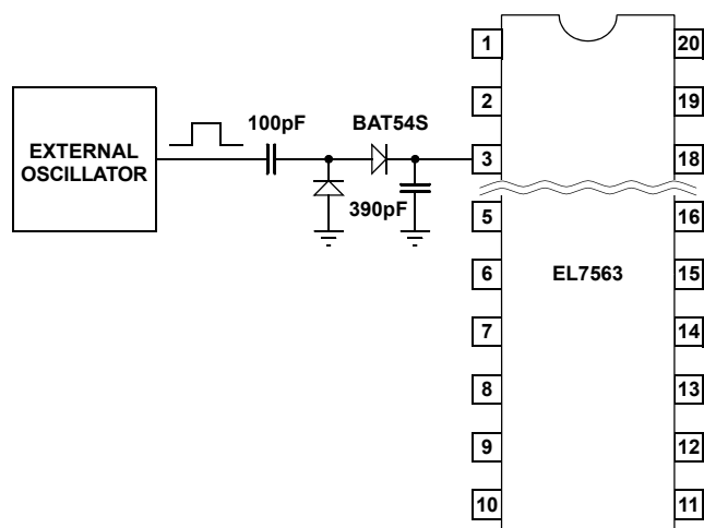
FIGURE 22. OSCILLATOR SYNCHRONIZATION
