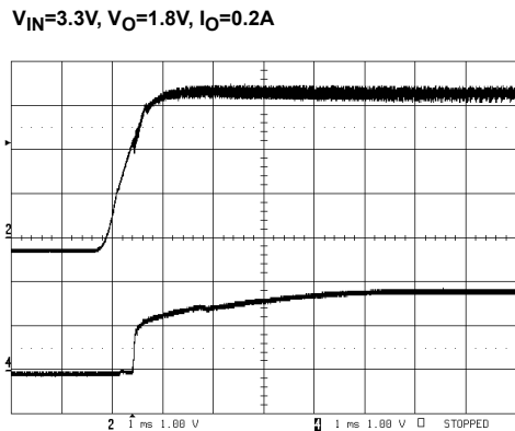
FIGURE 17. POWER-UP
