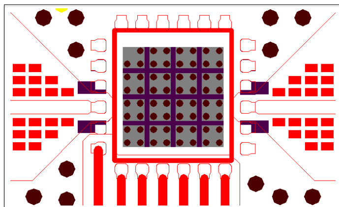
Via pattern
