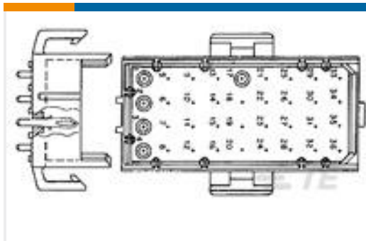
TE Part #640500-2 06P MR HDR ASSY V0
