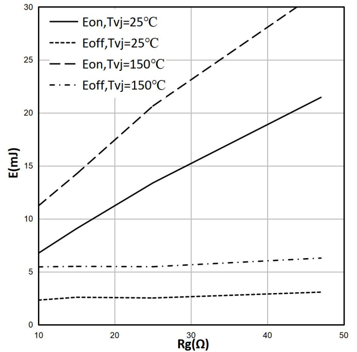
Figure 8. switching losses IGBT (typical)
