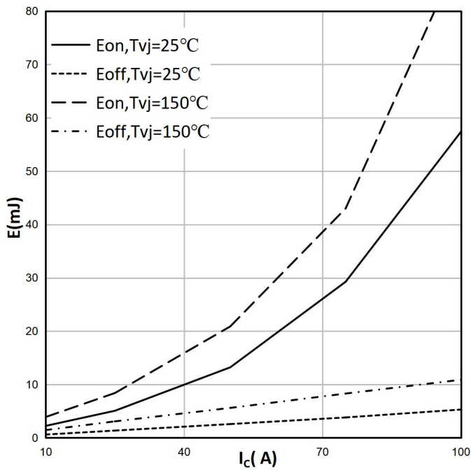
Figure7. switching losses IGBT (typical)
