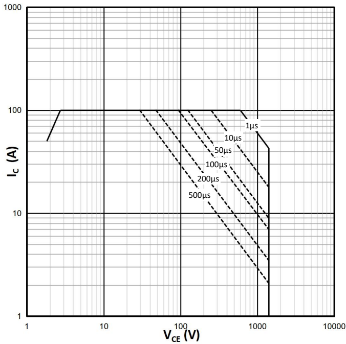
Figure5. FBSOA IGBT
