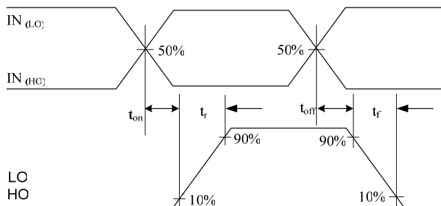
Figure 2: Switching Time Waveform Definitions
