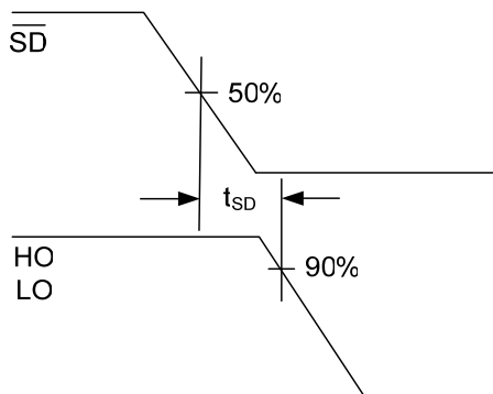
Figure 3: Delay Matching Waveform Definitions
