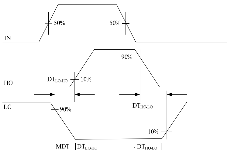
Figure 4: Deadtime Waveform Definitions
