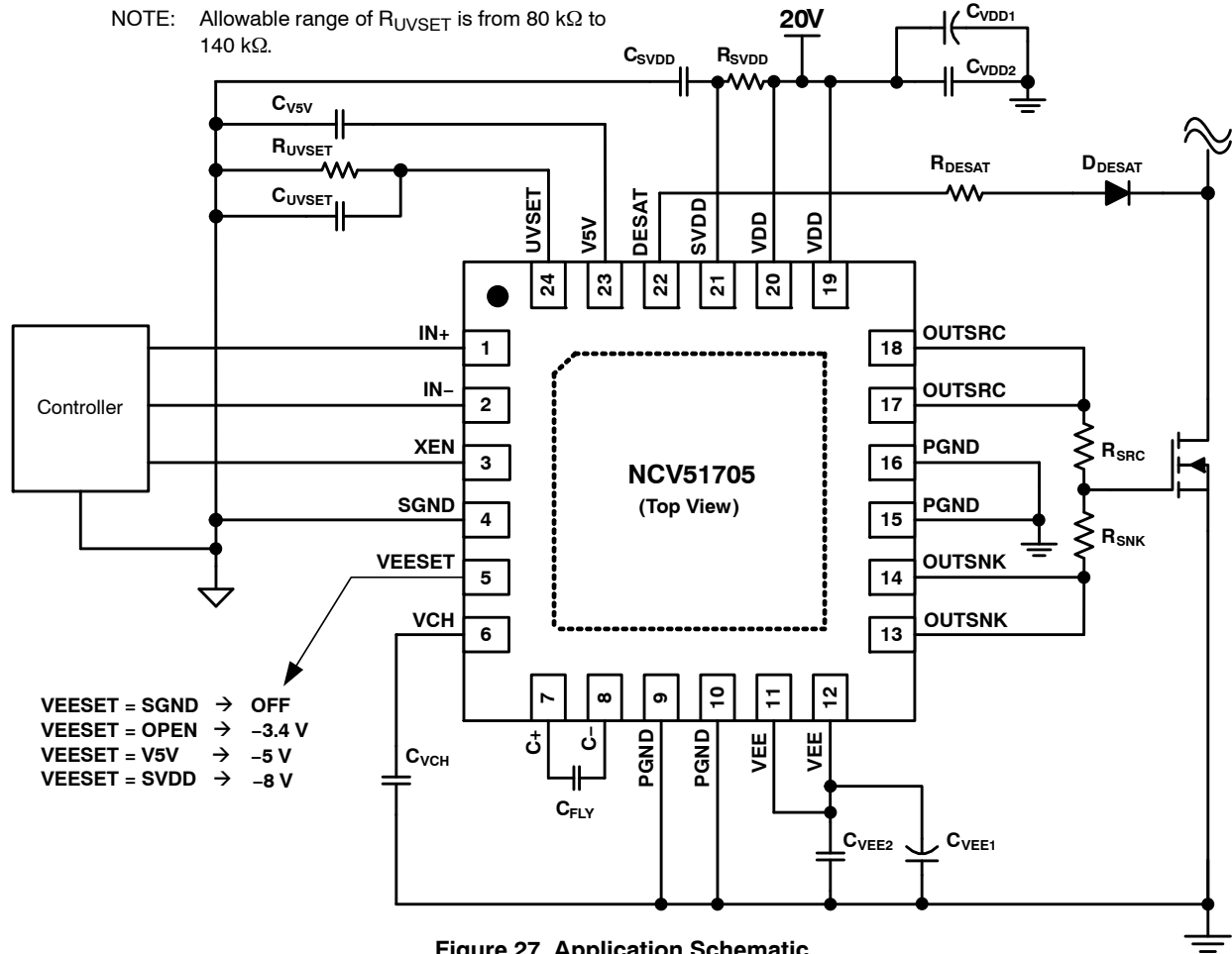
Figure 27. Application Schematic
