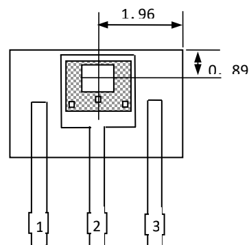
Sensor Location
