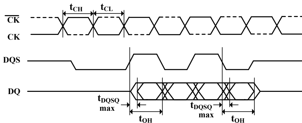
Figure 32. Data Output (Read) Timing
