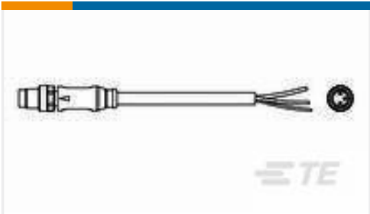
TE Part #2273000-1 M8 x 1.0 straight plug Pigtail
