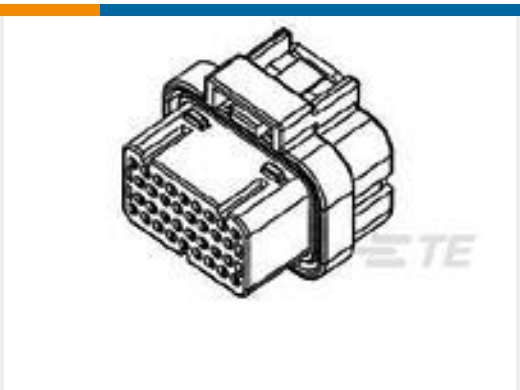
TE Part #4-1437290-0 34POS,SUPERSEAL,REC HSG ASSY, SLD,COD 1
