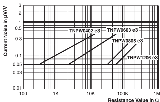
Current Noise
