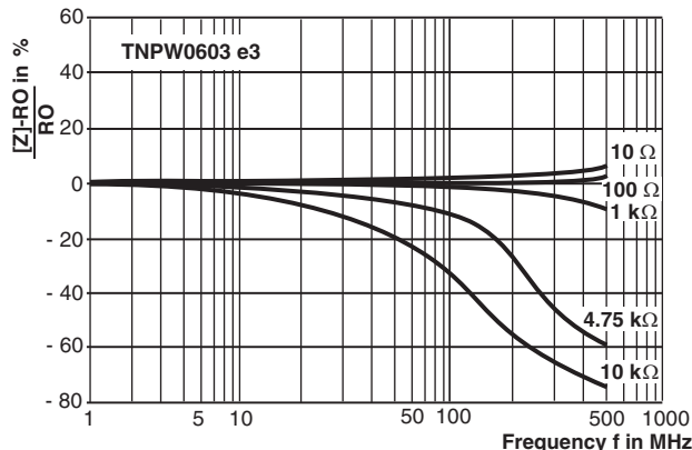
HF Performance (1)
