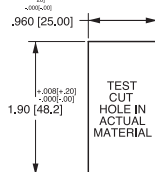
VMS MOUNTING PANEL HOLE
