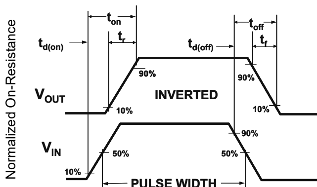
Figure 2: Switching Waveforms
