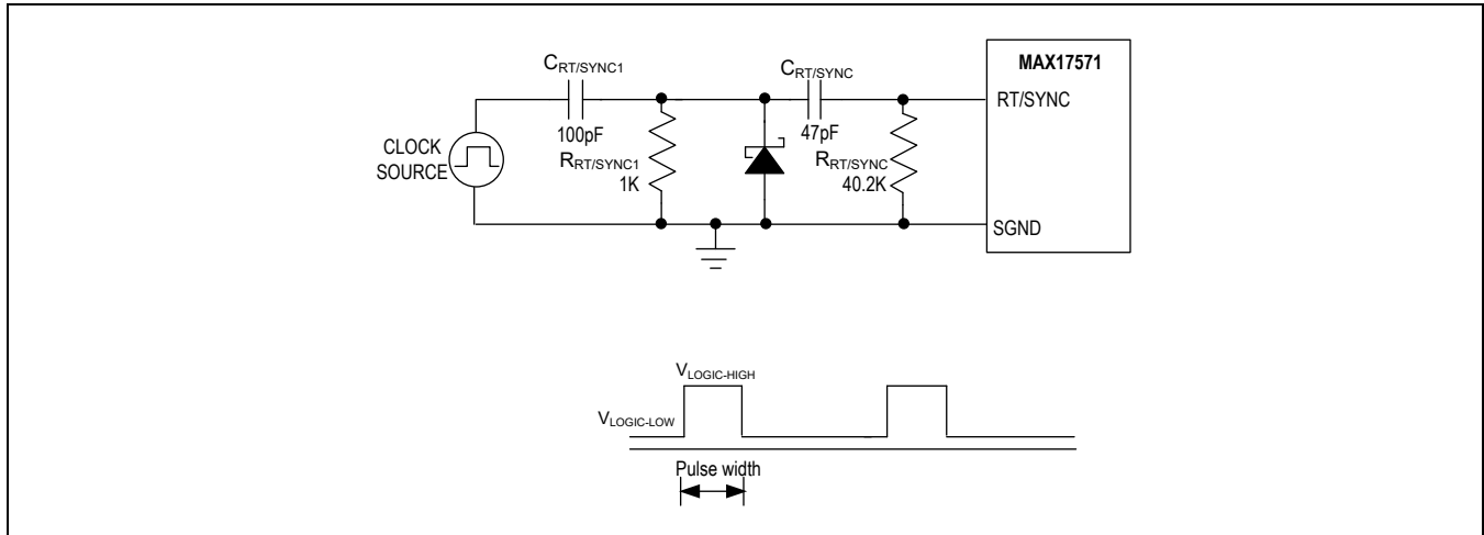
Figure 1. External Clock Synchronization
