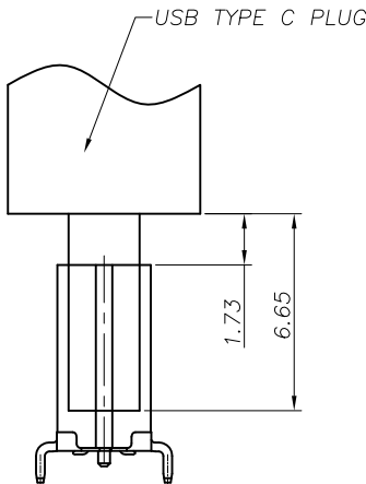
FEMALE AND MALE MATCHING DRAWING
