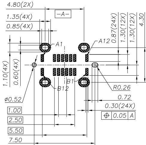
RECOMMENDED PCB LAYOUT(TOP VIEW) THICKNESS 0.8?.10MM;DEFAULT TOLERANCE:?.05
