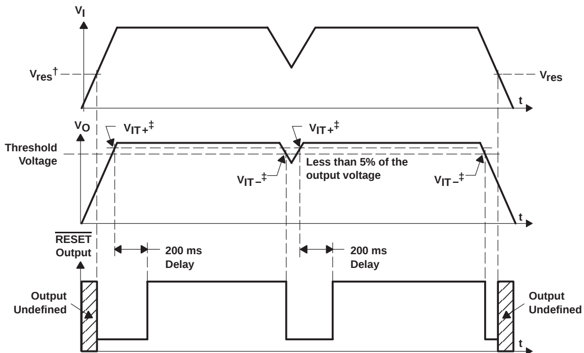
timing diagram
