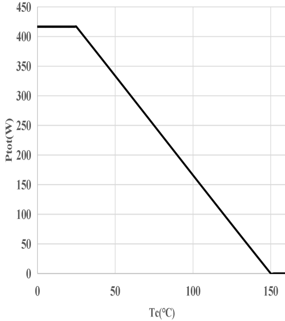
Figure 3: Power Dissipation
