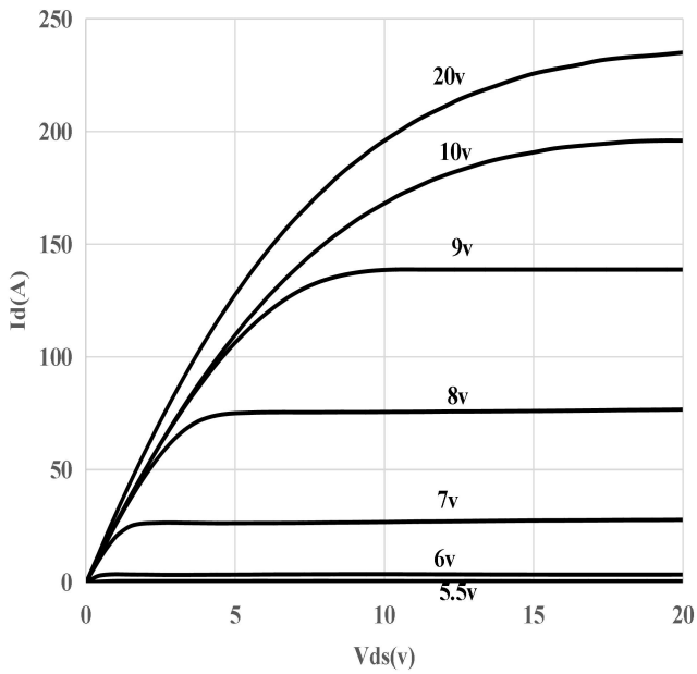
Figure 7: Typ. Output Characteristics
