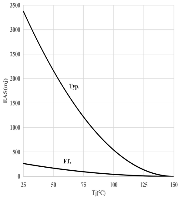
Figure 15: Avalanche Energy
