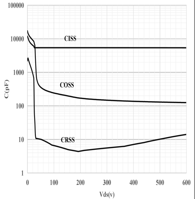
Figure 16: Typ. Capacitances
