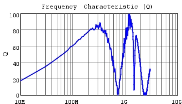
LQW2UASR27G0C Q
