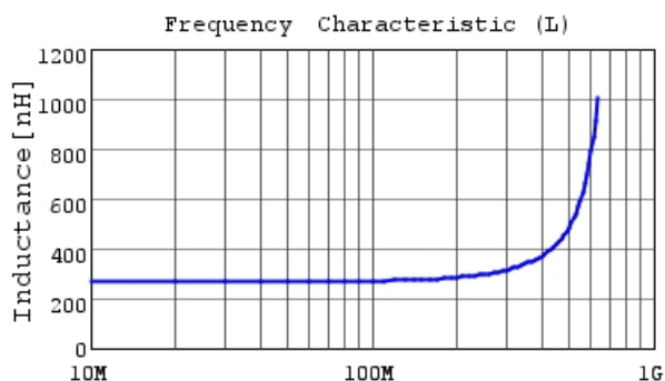
LQW2UASR27G0C L
