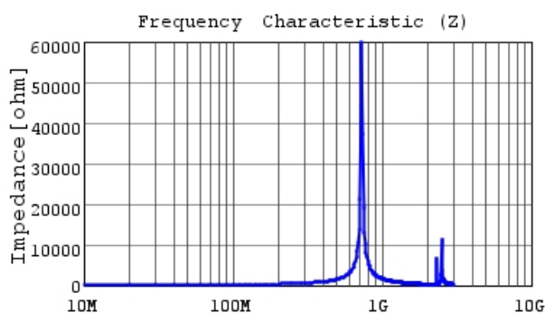
LQW2UASR27G0C |Z|
