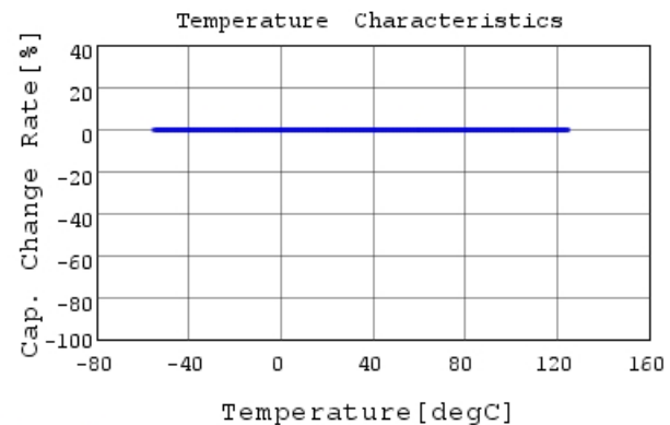
RCE5C2J222J1K1H03B C-Temp. capchange, DCOV,
