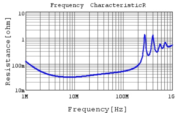
RCE5C2J222J1K1H03B R DCOV, 25degC
