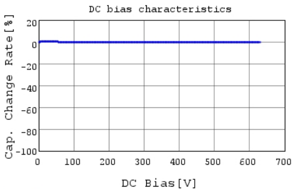
RCE5C2J222J1K1H03B C-DC bias capchange, 25.0
