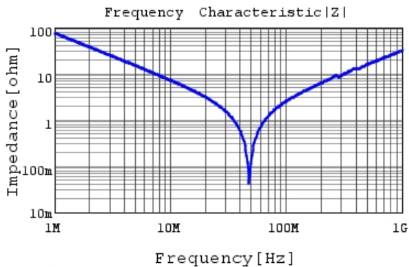
RCE5C2J222J1K1H03B |Z| DCOV, 25degC
