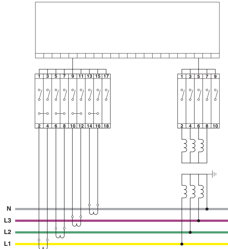
Circuit diagram
