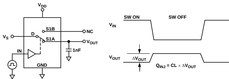
Figure 23. Charge Injection
