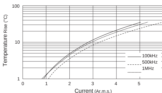
Ripple Current
