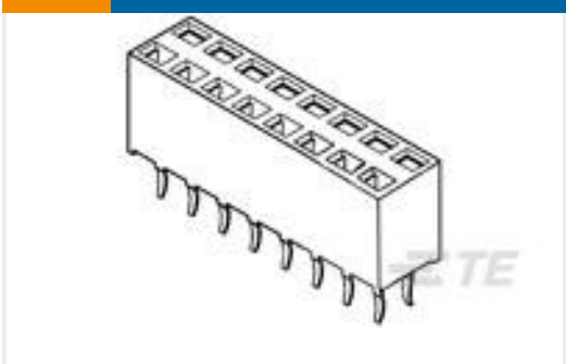
TE Part #215308-8 2X 8P HV100 REC CON. TE, 7.0MM, TIN
