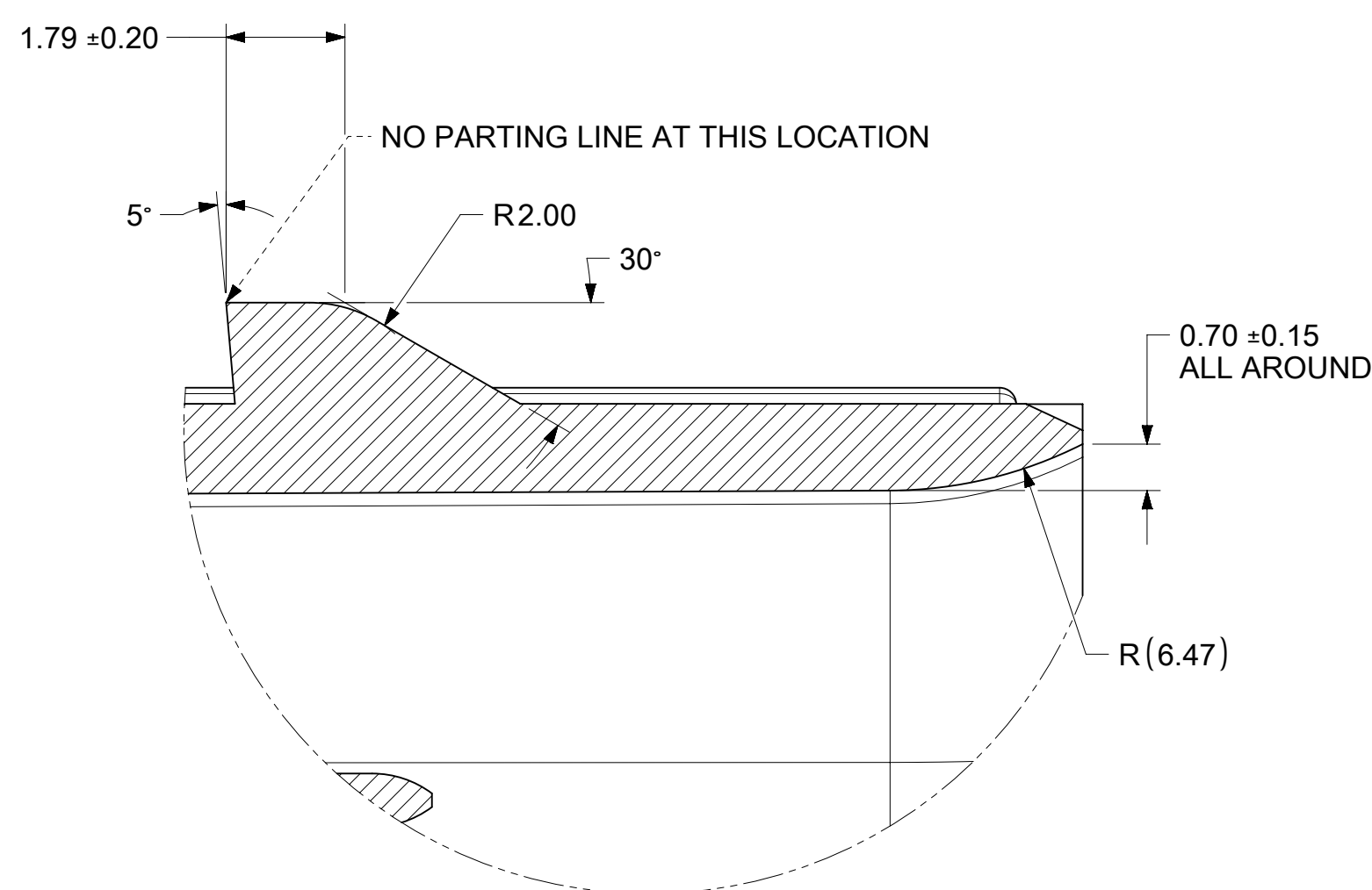
DETAIL 3 SCALE 10:1
