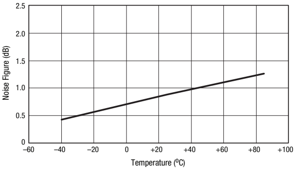
Figure 8. Noise Figure vs Temperature
