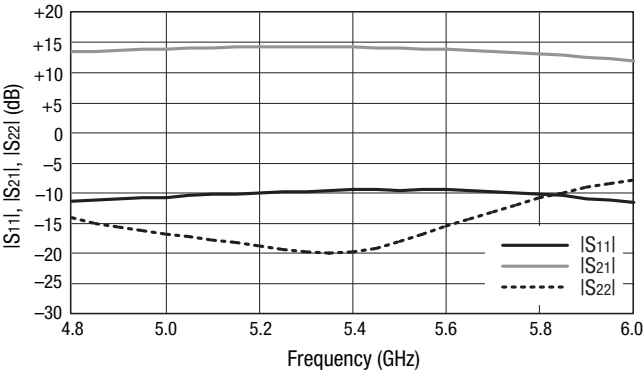
Figure 3. S-Parameter Data
