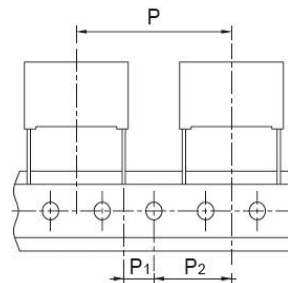
Lead Spacing 22.5 &amp; 27.5
