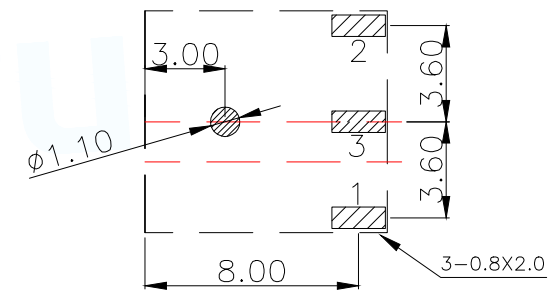
PCB.WELDING DRAWING (TOLERANCE:±0.05)
