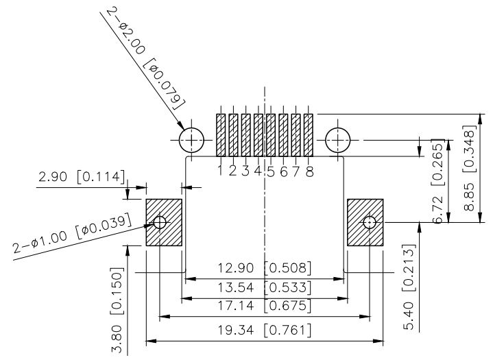
RECOMMENDED PCB LAYOUT VIEWED FROM COMPONENT SIDE
