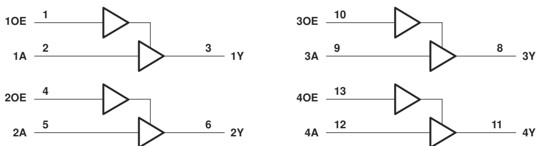
Figure 6-1. Logic Diagram (Positive Logic)
