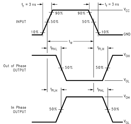
Figure 5. AC Waveforms
