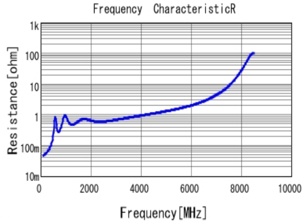
■ GRM1882C2A561JA01 R DC0V, 20degC
