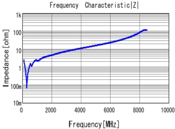
■ GRM1882C2A561JA01 |Z| DC0V, 20degC
