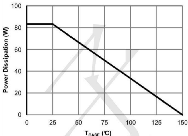
Figure 13: Power De-rating (Note F)
