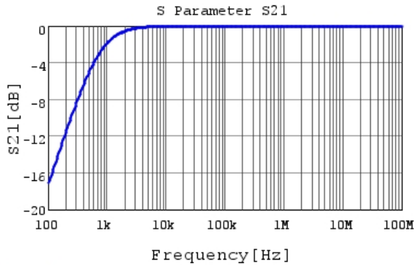
RHEL81E225K2K1H03B S21 DCOV, 25degC
