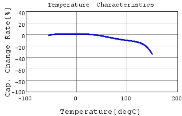
RHEL81E225K2K1H03B C-Temp. capchange, DCOV,
