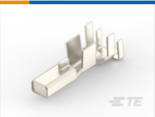
TE Part #1971781-1 Receptacle Contact — POWER TRIPLE LOCK
