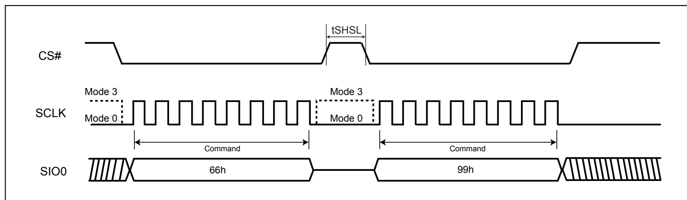
Figure 36. Reset Sequence
