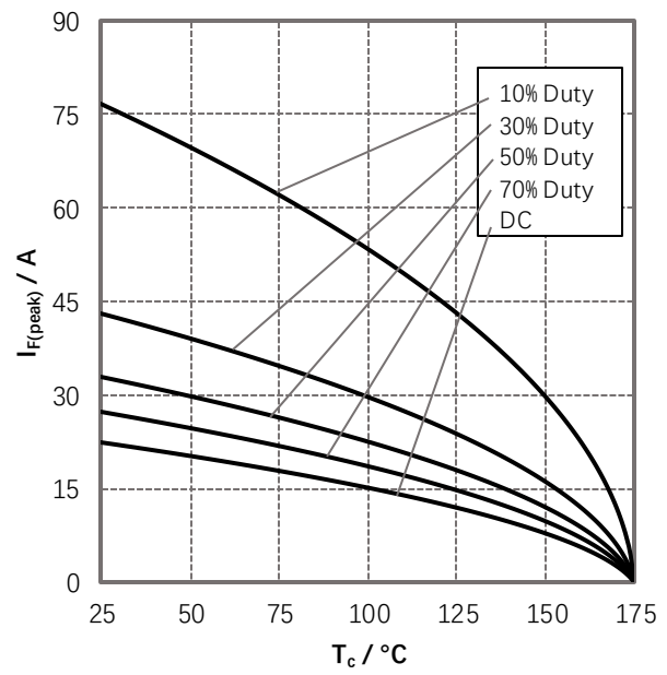
Figure 4. Current Derating
