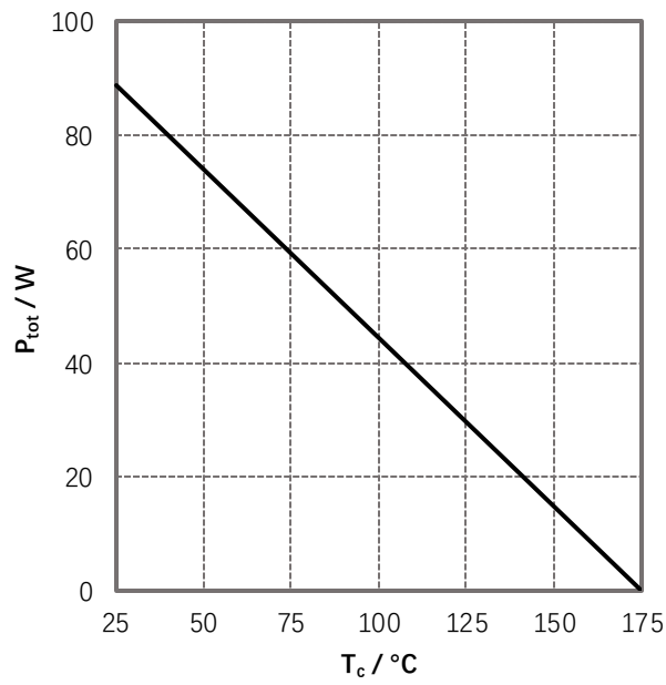
Figure 3. Power Derating
