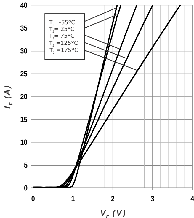
Figure 1. Forward Characteristics
