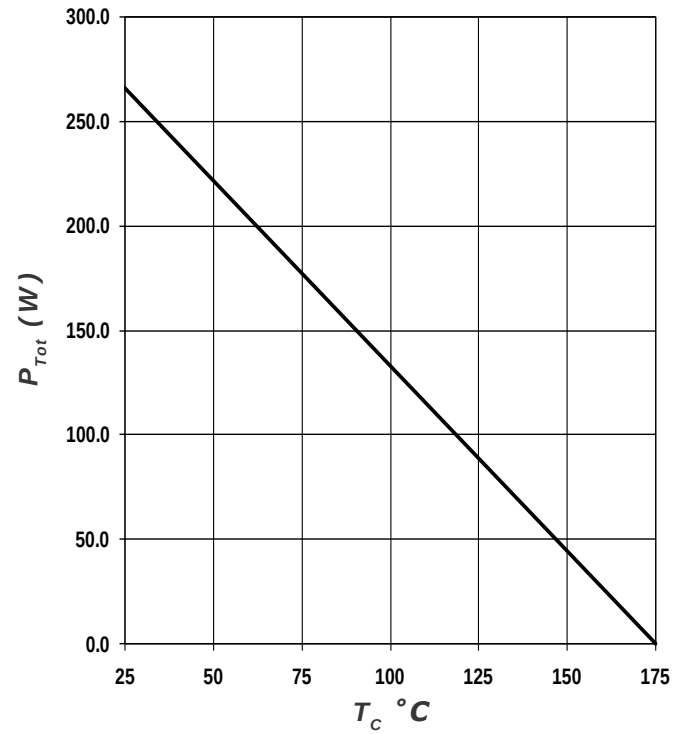
Figure 4. Power Derating
