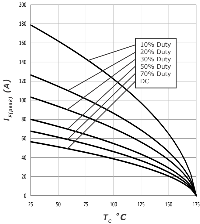
Figure 3. Current Derating
