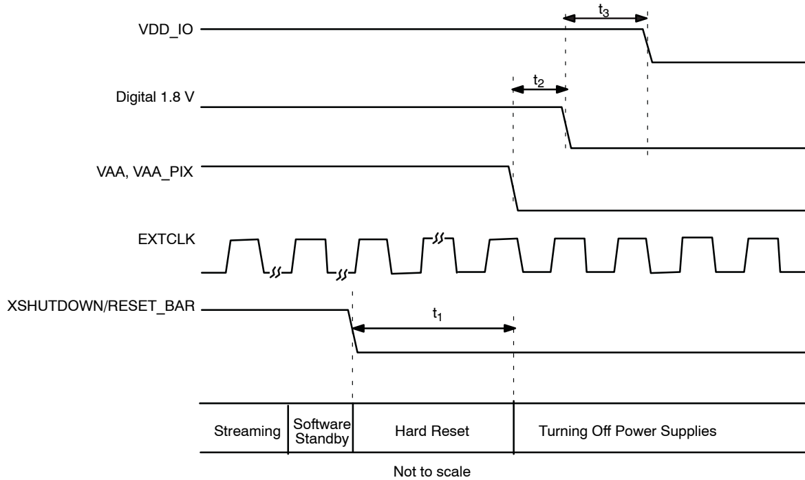
Figure 27. Power-Down Sequence
