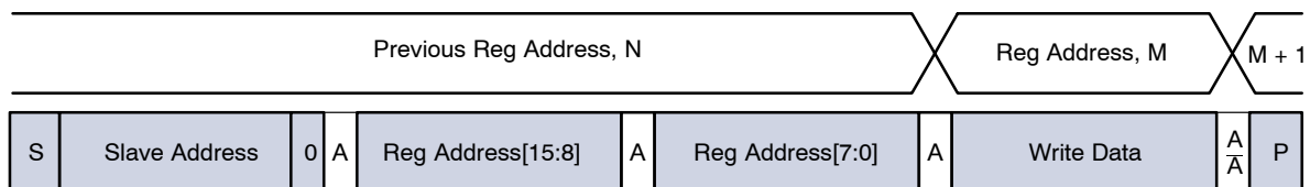
Figure 9. Single WRITE to Random Location
