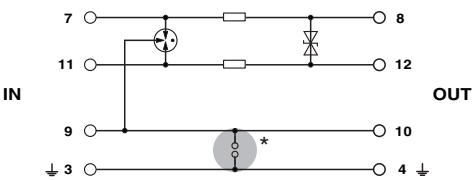
Circuit diagram
