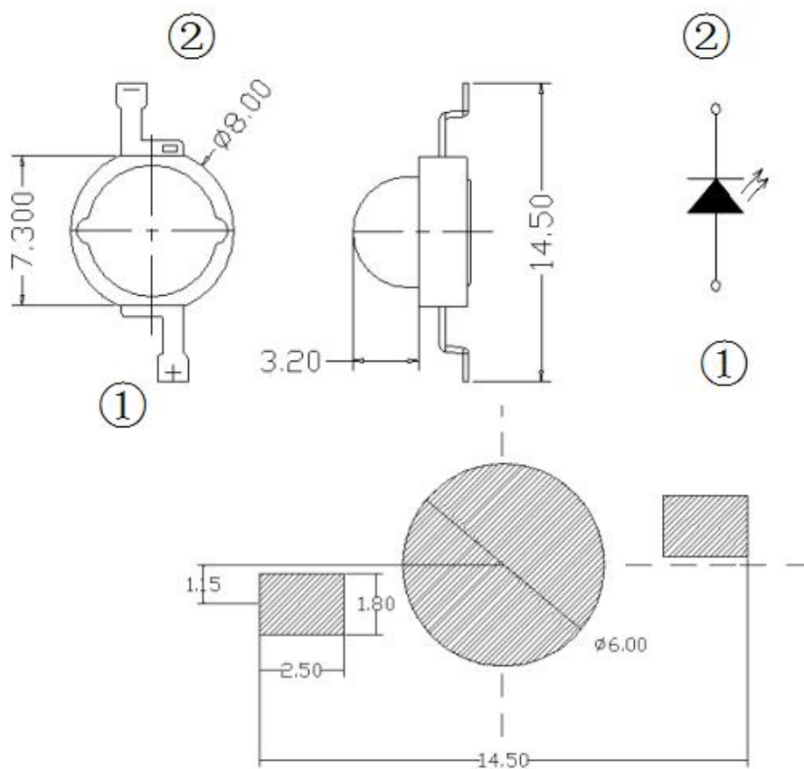
推荐焊盘 Recommmand soldering pad
