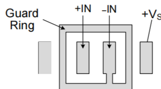
Figure4. Use guard ring around sensitive pins
