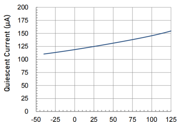
Temperature ( ^\circ\text{C} ) Quiescent Current as a function of Temperature.
