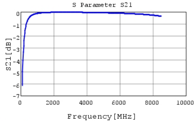
GRM0335C2A9R0WA01 S21 DCOV, 25degC
