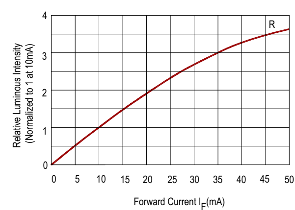
Figure 10: Relative Luminous Intensity vs. Forward Current
