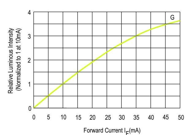
Figure 2: Relative Luminous Intensity vs. Forward Current
