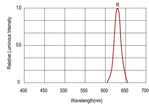
Figure 9: Relative Luminous Intensity vs. Wavelength
