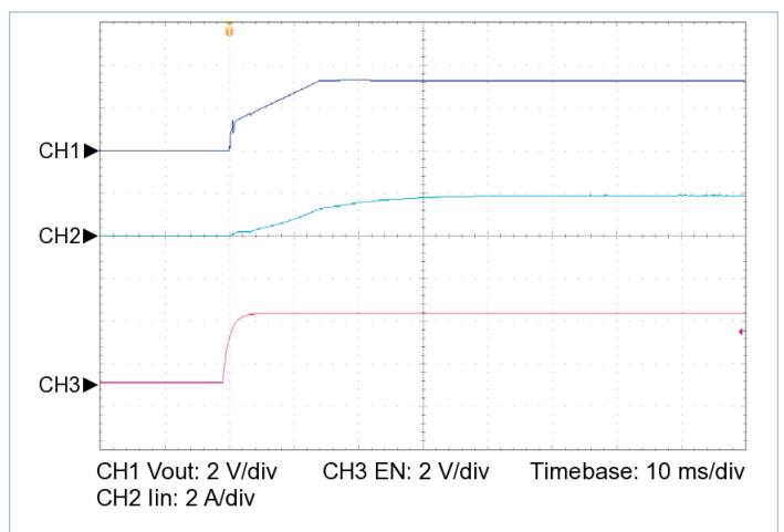
Figure 14 — Startup from EN, V_{IN} = 30\text{ V} , C_{OUT\_EXT} = 10000\text{ }\mu\text{F} , R_{LOAD} = 0.136\text{ }\Omega
