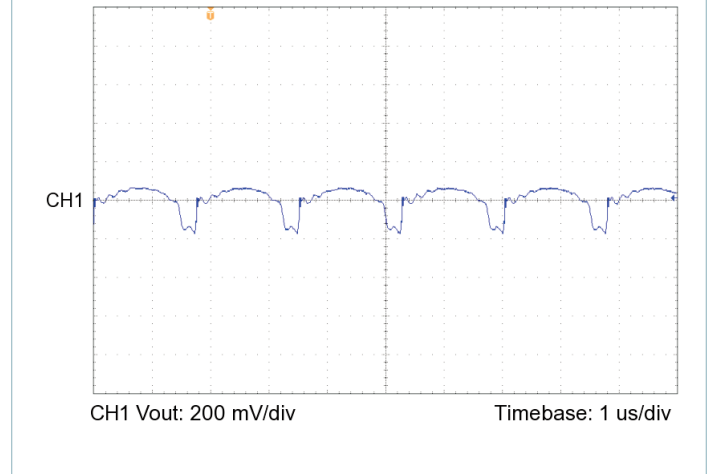
Figure 16 — Output voltage ripple, V_{IN} = 30\text{ V} , V_{OUT} = 3.3\text{ V} , C_{OUT\_EXT} = 1000\text{ }\mu\text{F} , R_{LOAD} = 0.136\text{ }\Omega
