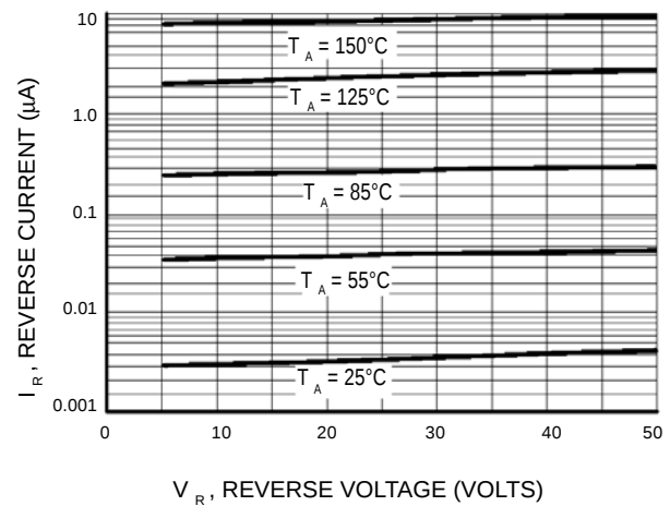
Figure 3. Leakage Current
