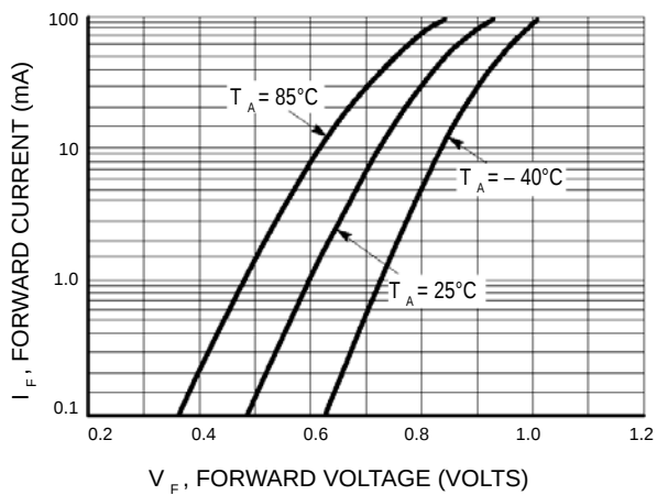
Figure 1. Forward Voltage
