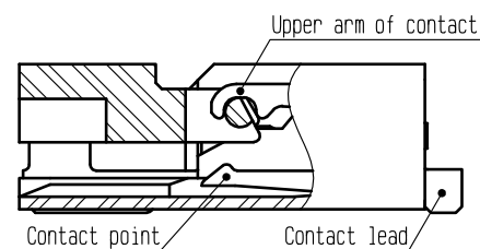
(Contact view)
