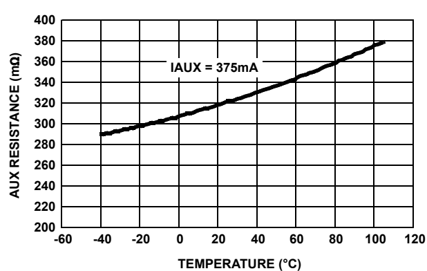
FIGURE 8. AUX r_{DS(ON)} vs TEMPERATURE
