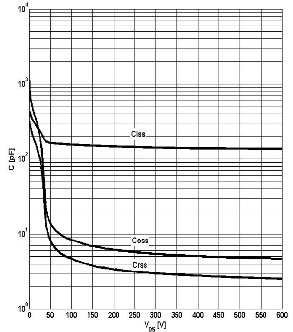
Figure 16: Typ. Capacitances
