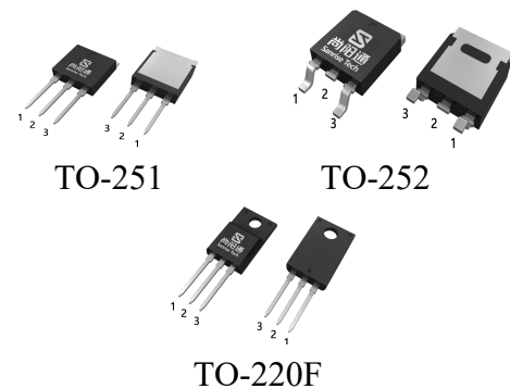
Figure 2 Package Types of SRC65R1K3ES
