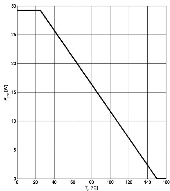
Figure 3: Power Dissipation
