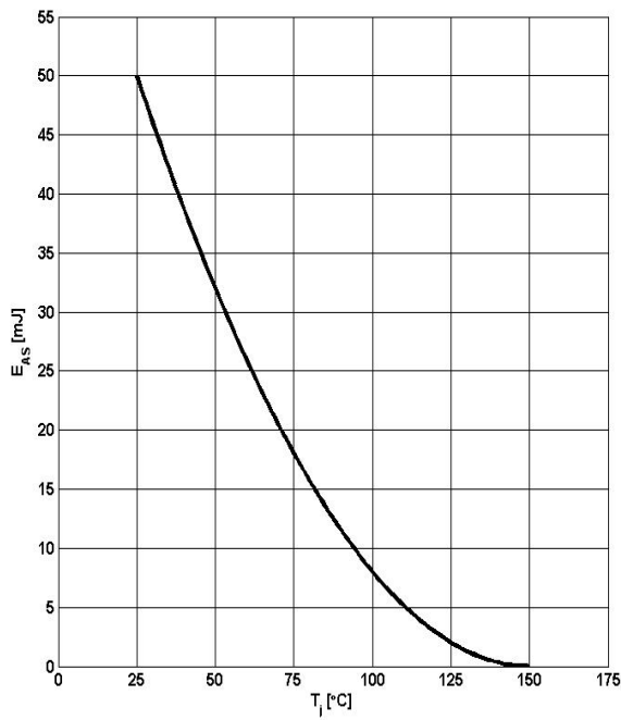
Figure 15: Avalanche Energy
